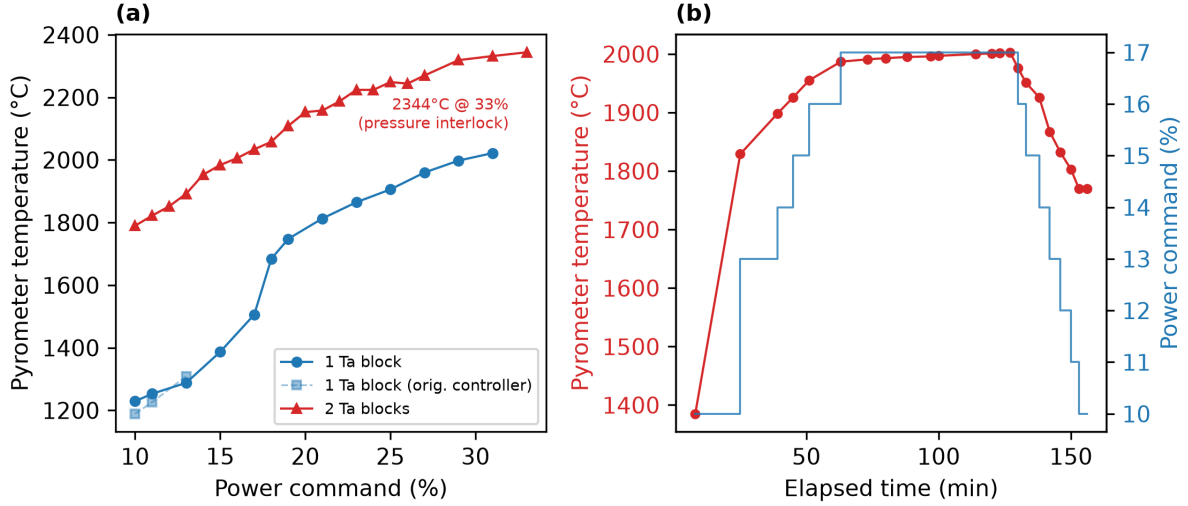
FIG. 16. Measured heat curves of the tantalum-susceptor (ceramic) stack (data contributed by R. Guymon). (a) Pyrometer temperature vs. generator power command for one and two stacked tantalum susceptor blocks (the faint series repeats the single-block measurement on the original power controller); the two-block ramp reached 2344 °C at a 33% command before the chamber pressure interlock ended the test. (b) Timed two-block ramp/soak: a constant 17% command holds \sim 2000 °C ( 2000 \pm 3 °C over the final hour) before a stepped ramp-down.
