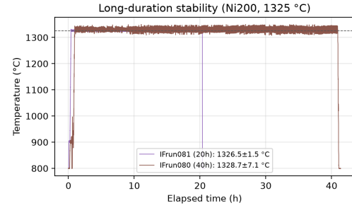
FIG. 11. Long-duration thermal stability: Ni200 anneals at 1325 °C held for 20 h (IFrun081) and 40 h (IFrun080).
