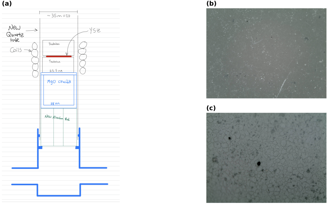
FIG. 15. High-temperature ceramic (YSZ) configuration and resulting microstructure. (a) Charge-stack schematic (contributed by R. Guymon): inside a fresh \sim 35 mm-ID quartz tube, the YSZ specimen (red) is sandwiched between two 25.5 mm tantalum susceptor blocks, seated in a 28 mm MgO crucible on an alumina support rod that raises the stack to coil height; the coil, vacuum, pyrometer, and control paths are unchanged from the metal configuration. (b) Optical micrograph of YSZ after a 1700 °C / 10 h anneal (docs/optical/.../190823_YSZ/YSZ.1700C.10h.JPG). (c) Optical micrograph of an induction-annealed YSZ specimen (docs/optical/.../190909_YSZ/), showing the equiaxed grain structure; scale-bar originals are inventoried in docs/optical/CATALOG.csv.
