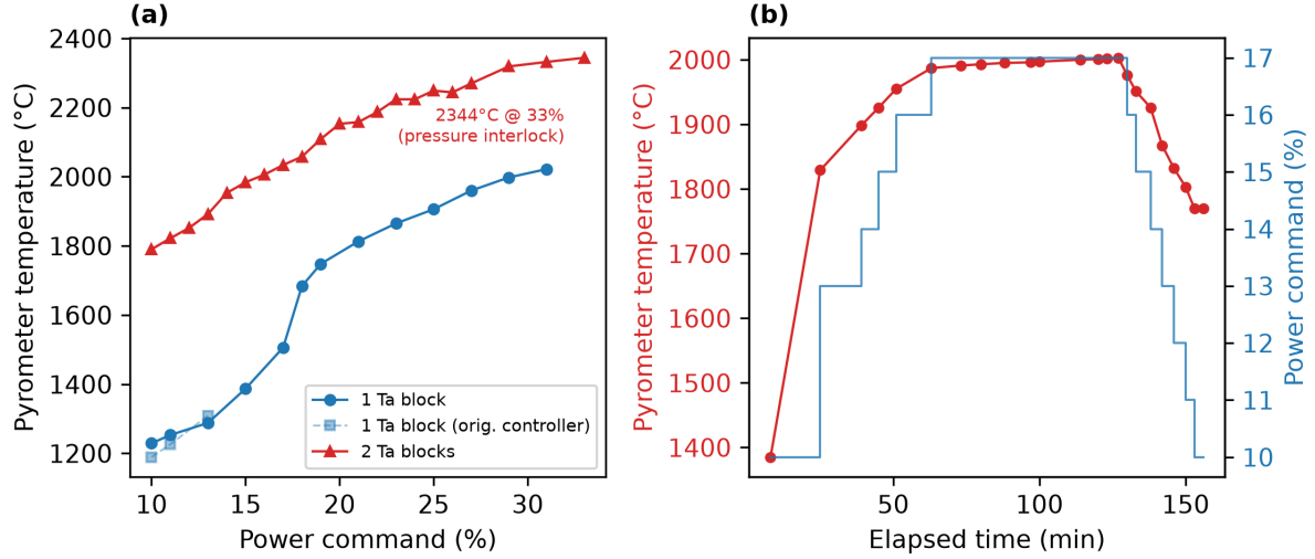
FIG. 14. Measured heat curves of the tantalum-susceptor (ceramic) stack, from the archived workbook docs/YSZ/Tantalum-Heat-Curve.xlsx (data contributed by R. Guymon). (a) Pyrometer temperature vs. generator power command for one and two stacked tantalum susceptor blocks (the faint series repeats the single-block measurement on the original power controller); the two-block ramp reached 2344 °C at a 33% command before the chamber pressure interlock ended the test. (b) Timed two-block ramp/soak: a constant 17% command holds \sim 2000 °C ( 2000 \pm 3 °C over the final hour) before a stepped ramp-down.
