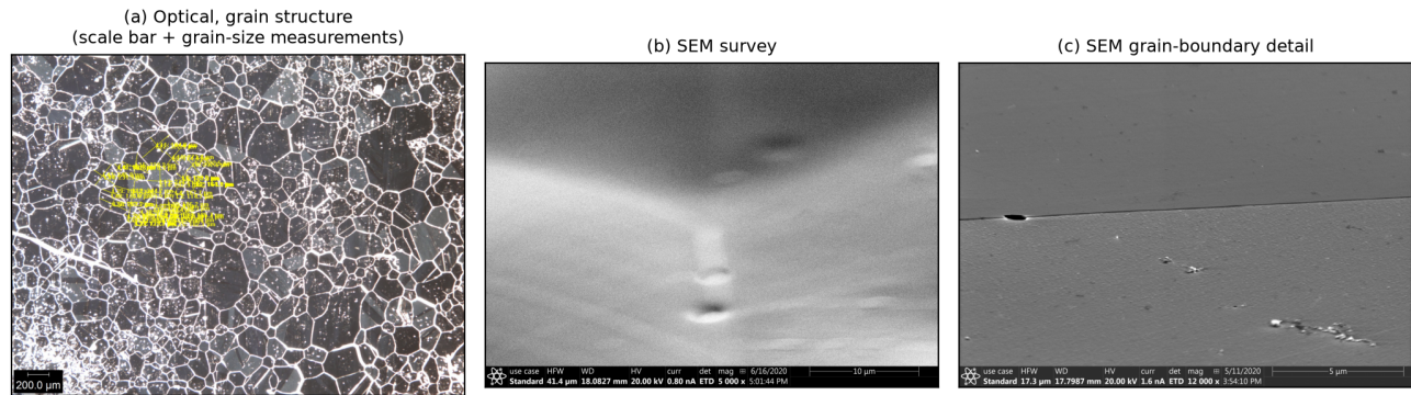
FIG. 13. Multi-scale microstructure of specimen Ni4N5_081 after IFRun082 (nominal 1300 °C / 20 h, gas flow), correlating the characterization archive with a single logged thermal history. (a) Optical micrograph (grain structure, 200 µm scale bar, with in-image grain-size measurements); (b) SEM survey; (c) high-magnification SEM grain-boundary detail. All panels are committed files under docs/optical/ and docs/SEM/ .
