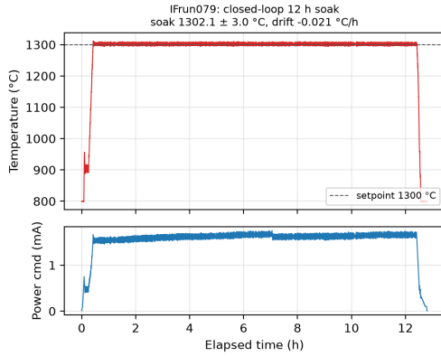
FIG. 9. Representative closed-loop anneal (IFrun079, Ni4N5, nominal 1300 °C / 12h): pyrometer temperature with setpoint overlay (top) and analog power command (bottom). Soak mean 1302.1 \pm 3.0 °C, drift -0.02 °C/h.
