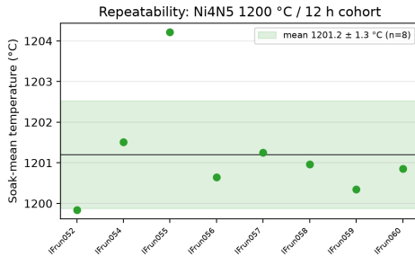
FIG. 10. Run-to-run repeatability of the Ni4N5 1200 °C / 12 h cohort (IFrun052–IFrun060, n = 8 ). Points are per-run soak-mean temperatures; the band is mean \pm SD ( 1201.2 \pm 1.3 °C).
