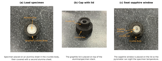
FIG. 3. Specimen-loading sequence for the graphite crucible/susceptor. (a) The specimen is placed between two alumina sheets in the crucible body. (b) The graphite lid is seated on top. (c) The sapphire window closes the lid bore, leaving an optical path for the pyrometer.
