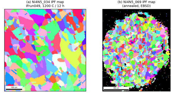
Figure 7: EBSD inverse-pole-figure (IPF) orientation maps of two annealed Ni4N5 specimens, rendered from the committed docs/SEM/ archive. (a) Ni4N5_034 (IFrun049, 1200 °C / 12 h); (b) Ni4N5_069. Each indexed color is a crystallographic orientation; the maps resolve hundreds of grains for grain-size and texture analysis.
