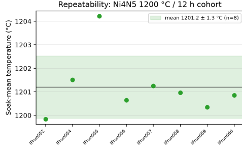
Figure 5: Run-to-run repeatability of the Ni4N5 1200 °C / 12h cohort (IFrun052–IFrun060, n = 8 ). Points are per-run soak-mean temperatures; the band is mean \pm SD ( 1201.2 \pm 1.3 °C).
