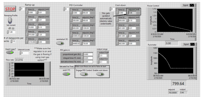
Figure 1: LabVIEW control front panel (docs/equipment-reference/frontPanel1.200219.PNG): editable ramp-up / PID-soak / cool-down setpoint tables (time vs. analog command in mA below the pyrometer floor and vs. °C once closed-loop), PID gains and output range, inert-gas flow setpoint/readback, and live power-command and pyrometer-temperature strip charts. Here the pyrometer reads ~800 °C during ramp.
