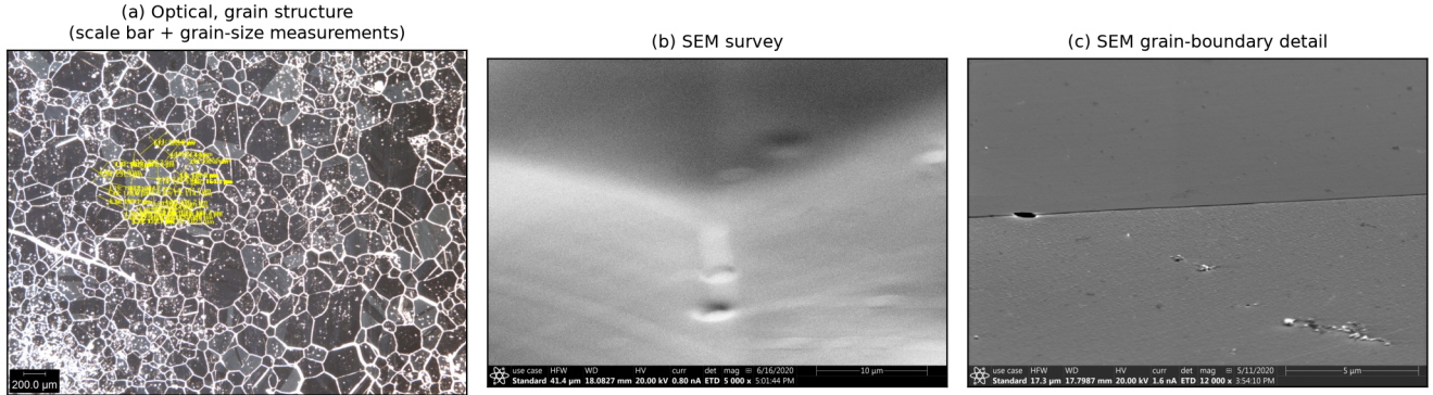
Figure 8: Multi-scale microstructure of specimen Ni4N5_081 after IFrun082 (nominal 1300 °C / 20 h, gas flow), correlating the characterization archive with a single logged thermal history. (a) Optical micrograph (grain structure, 200 µm scale bar, with in-image grain-size measurements); (b) SEM survey; (c) high-magnification SEM grain-boundary detail. All panels are committed files under docs/optical/ and docs/SEM/.
