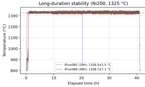
Figure 6: Long-duration thermal stability: Ni200 anneals at 1325 °C held for 20 h (IFrun081) and 40 h (IFrun080).
