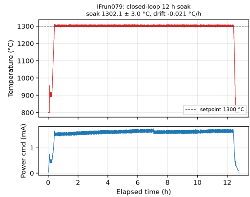
Figure 4: Representative closed-loop anneal (IFrun079, Ni4N5, nominal 1300 °C / 12 h): pyrometer temperature with setpoint overlay (top) and analog power command (bottom). Soak mean 1302.1 \pm 3.0 °C, drift -0.021 °C/h.
