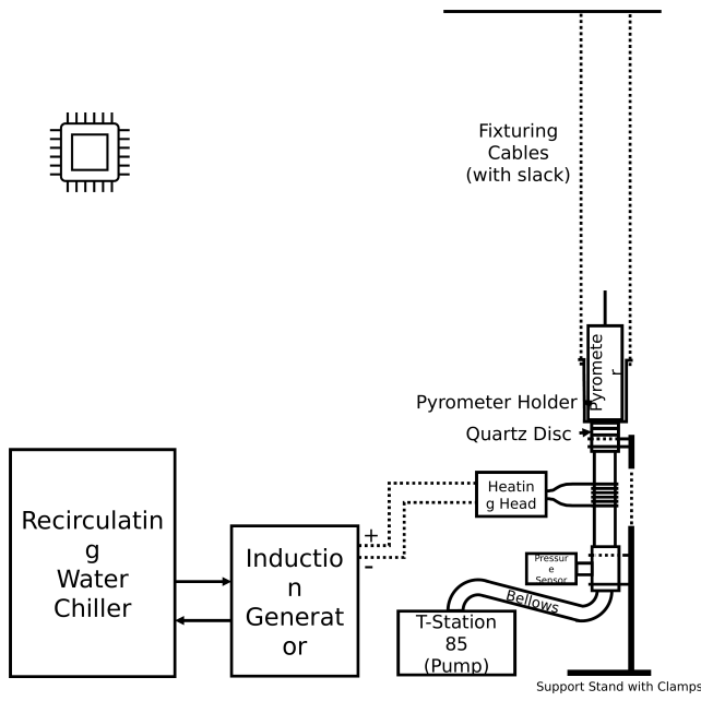
Figure 2: System overview of the computer-controlled, vacuum-integrated induction annealing system: recirculating water chiller and induction generator drive a water-cooled heating head/work coil around a quartz-tube vacuum chamber; a dual-wavelength pyrometer sights the charge through a quartz optical disc; an Edwards T-Station 85 turbo-molecular pump (with pressure gauge and bellows) evacuates the chamber; and a DAQ/laptop sets generator power and reads the pyrometer for closed-loop control. Rendered from the editable source schematic docs/induction-furnace-schematic.pptx.
