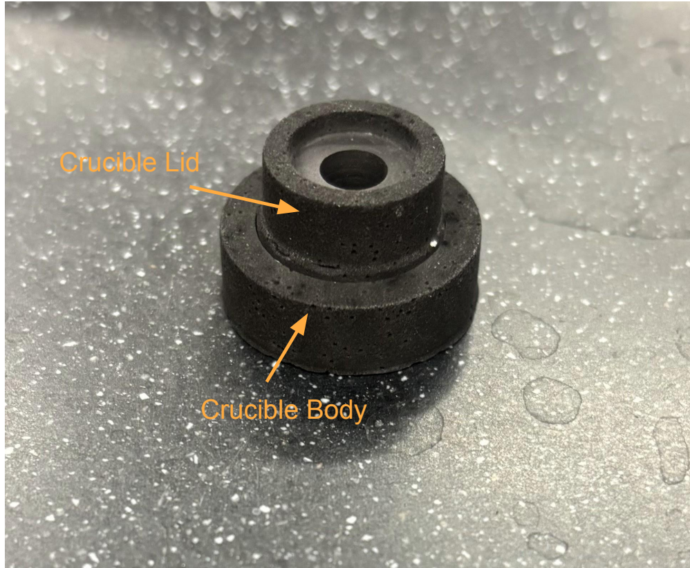
Caption: The lid is placed on top of the alumina-sample stack
