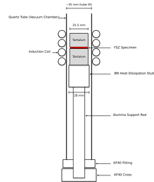
FIG. 8. Sample-stack configuration for the high-temperature ceramic anneals. The YSZ specimen is sandwiched between two 25.5mm tantalum susceptor blocks inside the quartz tube. The blocks rest on a boron nitride heat-dissipation stub, which sits on the alumina support rod that raises the sample stack to coil height. The coil, vacuum, pyrometer, and control paths are unchanged from the metal configuration.
