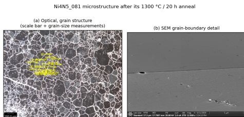
FIG. 5. Microstructure of specimen Ni4N5.081 after a 1300 °C / 20 h anneal under argon trickle flow. (a) Optical grain map with in-image grain-size measurements (200 \mu\text{m} scale bar); (b) high-magnification SEM grain-boundary detail.
