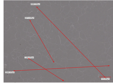
FIG. 7. As-recorded optical micrograph of the YSZ specimen after the 2500 ^{\circ}\text{C} / 45 min tantalum-susceptor anneal, which coarsened the grains from approximately 20 to 90 \mu\text{m} . The red traces are the microscope software's multi-grain size measurements (100 \mu\text{m} scale bar).
