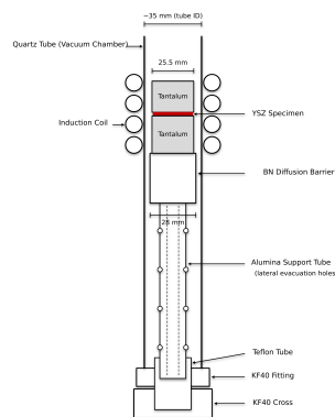
FIG. 8. Sample-assembly configuration for the high-temperature ceramic anneals. The YSZ specimen is sandwiched between two 25.5 mm tantalum susceptor blocks inside the quartz tube. The blocks rest on a boron nitride stub that acts as a diffusion barrier. It prevents reaction between the tantalum and the alumina support tube below, which raises the sample assembly to coil height. The alumina tube has holes bored laterally along its outer perimeter to aid evacuation, and a teflon tube couples its lower end to the KF40 fitting. The coil, vacuum, pyrometer, and control paths are unchanged from the metal configuration.
