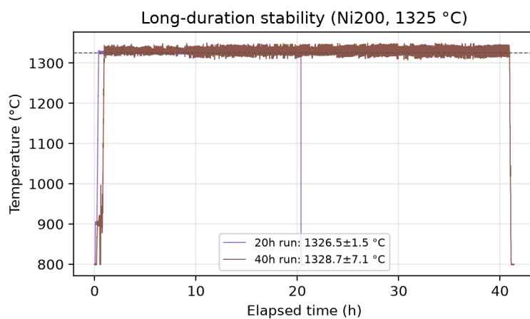
Figure S6: Long-duration thermal stability: Ni200 anneals at 1325 °C held for 20 h and 40 h.
