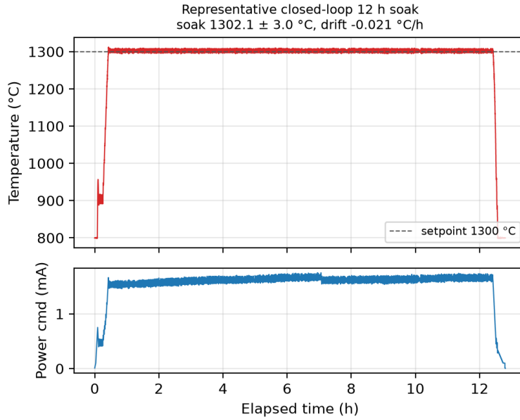
Figure S4: Representative closed-loop anneal (Ni 4 N 5 , nominal 1300 °C / 12 h): pyrometer temperature with setpoint overlay (top) and analog power command (bottom). Soak mean 1302.1 \pm 3.0 °C, drift -0.02 °C/h.
