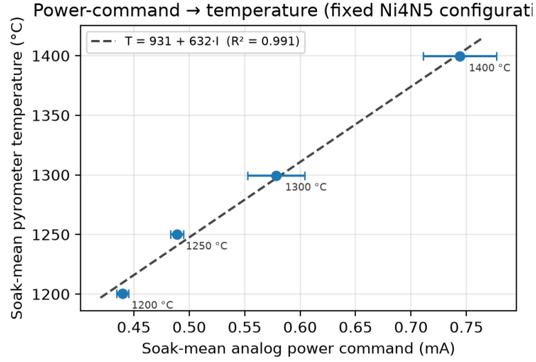
Figure S3: Power-command \rightarrow temperature calibration for one fixed Ni4N5 configuration. Points are soak-mean values; horizontal bars are the in-soak standard deviation of the analog command. The dashed line is the linear operational calibration ( R^2 = 0.991 , n = 4 ).
