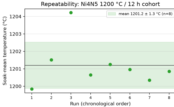
Figure S5: Repeatability of the Ni 4 N 5 1200 °C / 12 h cohort ( n = 8 ). Points are per-run soak-mean temperatures; the band is mean \pm SD ( 1201.2 \pm 1.3 °C).
