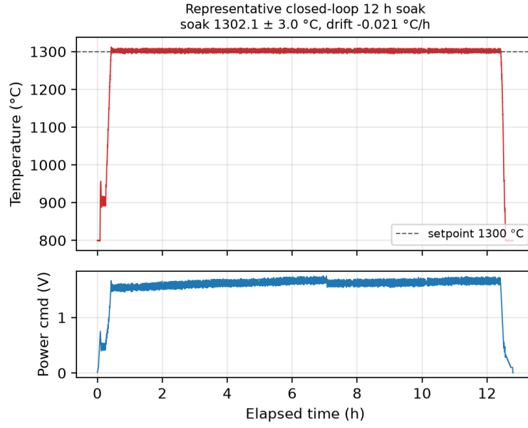
Figure S5: Representative closed-loop anneal (Ni (4N5), nominal 1300 °C / 12 h): pyrometer temperature with setpoint overlay (top) and power command in volts on the DAQ's 0–5 V scale (bottom; the soak-mean command of 1.6 V corresponds to approximately 32 % of full scale). Soak mean 1302.1 \pm 3.0 °C, drift -0.02 °C/h.
