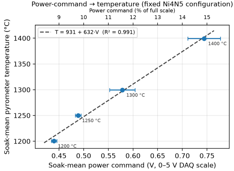
Figure S4: Power-command \rightarrow temperature calibration for one fixed Ni (4N5, i.e., 99.995 % purity) configuration. The command is expressed in volts on the DAQ's 0–5 V analog-output scale (top axis: the equivalent percent of full scale). Points are soak-mean values; horizontal bars are the in-soak standard deviation of the command. The dashed line is the linear operational calibration ( R^2 = 0.991 , n = 4 ).
