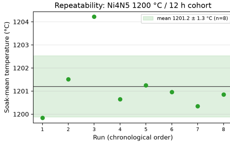
Figure S6: Repeatability of the Ni (4N5) 1200 °C / 12 h cohort ( n = 8 ). Points are per-run soak-mean temperatures; the band is mean \pm SD ( 1201.2 \pm 1.3 °C).
