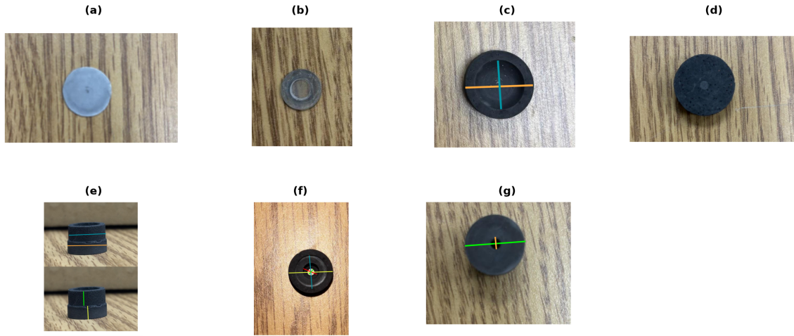
Figure S1: Measured dimensions of each part of the graphite crucible/susceptor assembly; each dimension is keyed to the color of the measurement line drawn on the photograph. (a) Alumina spacer disc, 14 mm dia. (b) Sapphire pyrometer window, 9.5 mm dia., 0.5 mm thick. (c) Crucible body, top: machined sample cavity 14.55 mm ID (teal) and 20.30 mm OD (orange); the cup is 6.5 mm tall with a 2 mm base. (d) Crucible body, bottom face, 20.30 mm dia. (e) Crucible lid, oblique, with the stepped plug that seats into the cavity: 13.70 mm upper-step diameter (teal) and 14.55 mm lower-shoulder diameter (orange); the upper step is 6 mm tall (green) and the lower shoulder 4 mm tall (yellow). (f) Crucible lid, top: 13.70 mm outermost diameter (yellow), 9.75 mm second step (teal), 5 mm third step (red), and the 3.5 mm central pyrometer-sighting bore (green). (g) Crucible lid, bottom: 14.55 mm seating face (green) and the 3.5 mm through-bore (orange). Fully assembled the crucible stands 13 mm tall.
