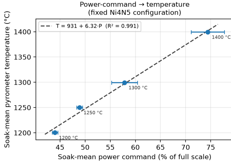
Figure S4: Power-command → temperature calibration for one fixed Ni (4N5, i.e., 99.995 % purity) configuration. The command is expressed as a percentage of the generator's full scale. Points are soak-mean values; horizontal bars are the in-soak standard deviation of the command. The dashed line is the linear operational calibration ( R^2 = 0.991 , n = 4 ).
