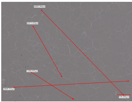
FIG. 7. As-recorded optical micrograph of a YSZ specimen after the 2500 °C / 45 min tantalum-susceptor anneal, which coarsened the grains from approximately 20 to 90 μm. The red traces are the microscope software’s multi-grain size measurements (100 μm scale bar).
