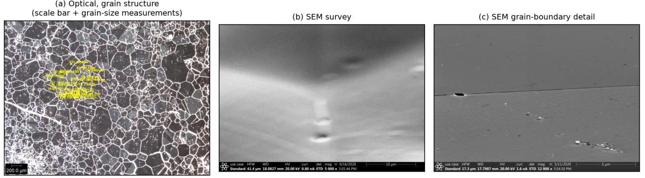
FIG. 14. Multi-scale microstructure of specimen Ni4N5_081 after IFrun082 (nominal 1300 °C / 20 h, gas flow), correlating the characterization archive with a single logged thermal history. (a) Optical micrograph (grain structure, 200 µm scale bar, with in-image grain-size measurements); (b) SEM survey; (c) high-magnification SEM grain-boundary detail.
