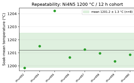
FIG. 11. Run-to-run repeatability of the Ni4N5 1200 °C / 12 h cohort (IFrun052–IFrun060, n = 8 ). Points are per-run soak-mean temperatures; the band is mean \pm SD ( 1201.2 \pm 1.3 °C).
