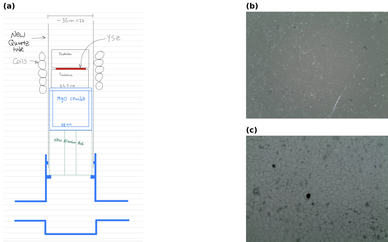
FIG. 16. High-temperature ceramic (YSZ) configuration and resulting microstructure. (a) Charge-stack schematic (contributed by R. Guymon): inside a fresh \sim 35 mm-ID quartz tube, the YSZ specimen (red) is sandwiched between two 25.5 mm tantalum susceptor blocks, seated in a 28 mm MgO crucible on an alumina support rod that raises the stack to coil height; the coil, vacuum, pyrometer, and control paths are unchanged from the metal configuration. (b) Optical micrograph of YSZ after a 1700^\circ\text{C} / 10 h anneal. (c) Optical micrograph of an induction-annealed YSZ specimen, showing the equiaxed grain structure.
