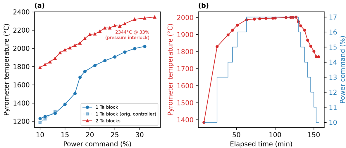
FIG. 15. Measured heat curves of the tantalum-susceptor (ceramic) stack (data contributed by R. Guymon). (a) Pyrometer temperature vs. generator power command for one and two stacked tantalum susceptor blocks (the faint series repeats the single-block measurement on the original power controller); the two-block ramp reached 2344 °C at a 33% command before the chamber pressure interlock ended the test. (b) Timed two-block ramp/soak: a constant 17% command holds \sim 2000 °C ( 2000 \pm 3 °C over the final hour) before a stepped ramp-down.
