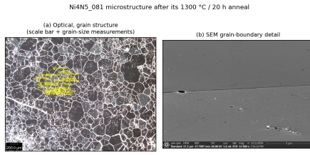
FIG. 9. Microstructure of a Ni4N5 specimen after a 1300 °C / 20 h anneal under a constant 20SCCM argon flow. (a) Optical grain map with in-image grain-size measurements (200 \mu\text{m} scale bar); (b) high-magnification SEM grain-boundary detail.
