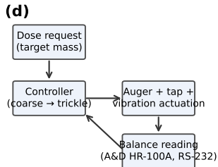
Closed-loop gravimetric dosing
