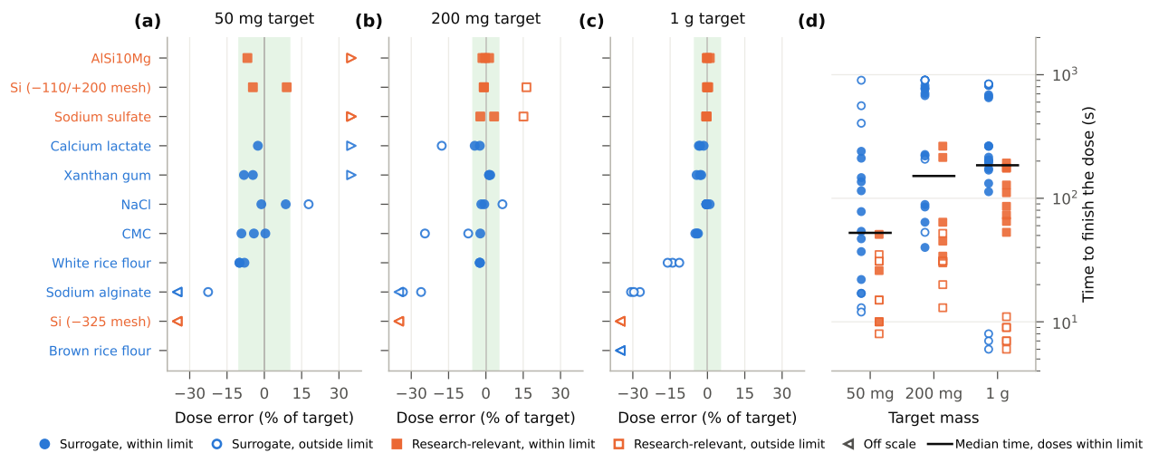
Fig. 5 Closed-loop dosing with one frozen set of controller settings. (a–c) Error of each valid dose at 50 mg, 200 mg and 1 g targets, as a percentage of the target. Green bands mark the acceptance limits ( \pm 10\% below 100 mg, \pm 5\% at or above). Filled markers finished within the limit and open markers outside it; triangles at the edge are off scale (the powders that delivered little or nothing). Replicates share a row and are not jittered. Powders are ordered by mass per revolution (Fig. 3a). Doses at 1 g for the food-safe powders are from the first test round (protocol G, August 2026); all 50 and 200 mg doses and the 1 g doses for AISi10Mg, coarse silicon, and sodium sulfate are from the second round (protocols G and H, September 2026). Barium chloride has no valid closed-loop dose (it caked in the tube) and fumed silica was not dosed. (d) Time to finish each dose; horizontal bars are medians of the doses within the limit.
