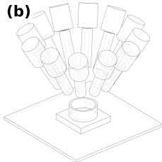
Inward-tilting channels over shared cup (preliminary CAD)
