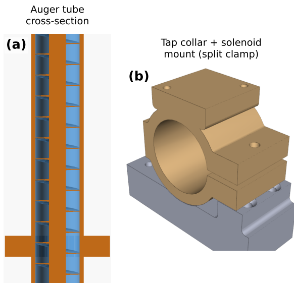
Fig. 2 Design specifics. (a) Cross-section of the printed auger tube showing the helical channel and flight clearances. (b) Split-clamp tap collar designed to carry the solenoid striker and ERM vibration motor; the clamp couples impacts into the powder column without loading the auger bearing.
