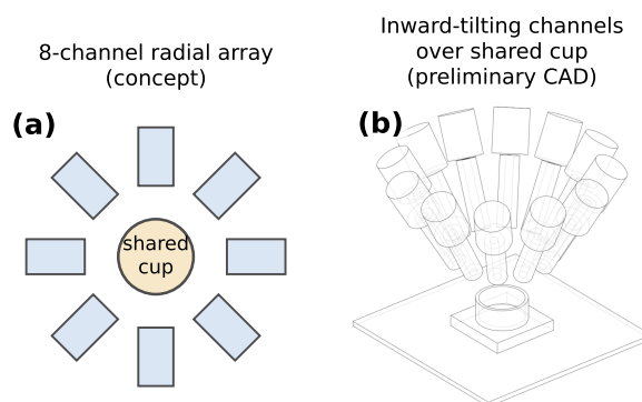
Fig. 5 Future work: multi-powder doser. (a) Eight-channel radial array concept around a shared collection cup. (b) Preliminary CAD study of inward-tilting channels over the shared cup.
