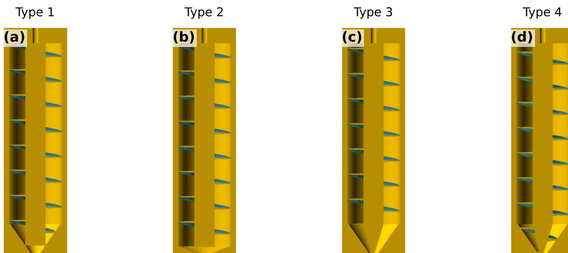
Figure S1: Cross-sections of the four exit-nozzle variant CAD models (Types 1–4, panels (a)–(d)) of the test auger, differing in exit constriction and chamfer geometry.
