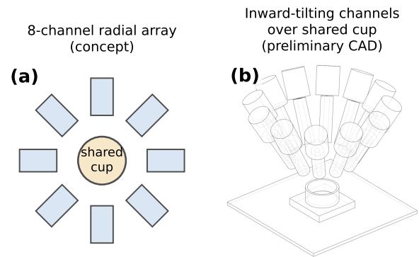
Fig. 5 Future work: multi-powder doser. (a) Eight-channel radial array concept (schematic) around a shared collection cup. (b) Preliminary programmatic-CAD study of inward-tilting channels over the shared cup. As elsewhere, the concept was set by the human team and the CAD modelled by AI coding agents; no GUI CAD package was used.
