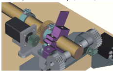
17. Tap-collar clamp [6, 22]
