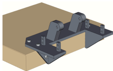
6. Mounting plate on the hinge [9]
