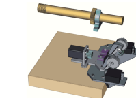
16. Bracket screws and clamps [5, 6, 22]
