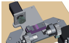
14. Auger onto the plate [19-21]
