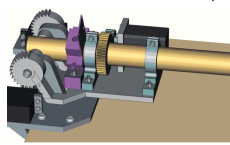
16. Bracket screws and clamps [5, 6, 22]
