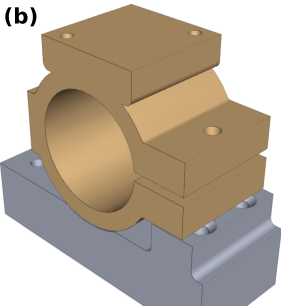
Tap collar + solenoid mount (split clamp)
