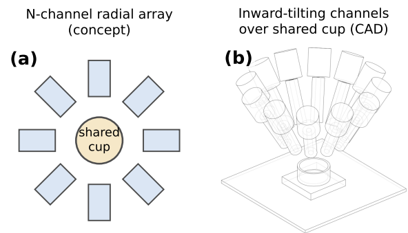
Fig. 5 Future work: multi-powder doser. (a) N -channel radial array concept around a shared collection cup on a single balance. (b) CAD study of inward-tilting channels over the shared cup.
