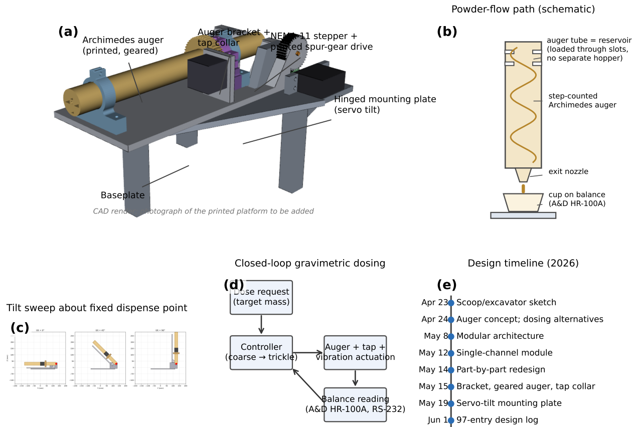
Fig. 1 Platform overview. (a) Single-channel powder-doser module (CAD render; photograph of the printed platform will replace this render): printed Archimedes auger, printed spur-gear drive from a NEMA-11 stepper, tap collar carrying the solenoid striker and ERM vibration motor, and servo-tilted hinged mounting plate on the baseplate. (b) Schematic of the powder-flow path through the module: powder is loaded through slots into the auger tube, which is itself the reservoir (no separate hopper), and is conveyed down the helical channel → exit nozzle → collection cup on the analytical balance. (c) Tilt sweep about the fixed dispense point: the hinge axis passes through the exit-nozzle tip so the dispense point does not translate as the channel tilts from 0° (horizontal park) to 90° (vertical dispense). (d) Closed-loop gravimetric dosing concept: the target mass enters the controller, which drives the actuation while the balance feeds the measured mass back. (e) Compressed design timeline; the complete 97-entry design log is available in the repository.
