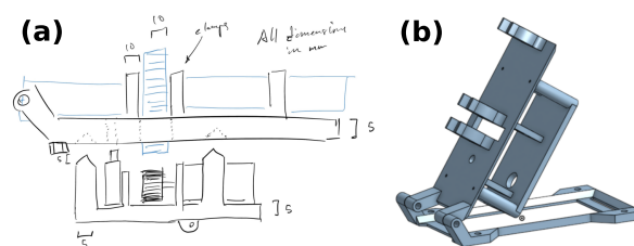
Fig. 6 Future work: the multi-powder doser, in which passive auger cartridges ride on a roller chain past one fixed station that turns, taps and weighs them (repository issue #128). (a) Hand sketch of the auger carriage, drawn before modelling (dimensions in mm). (b) The auger and frame carriages of the first printed prototype, modelled by the team in Onshape, a conventional CAD package.
