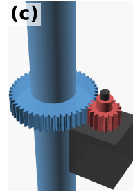
Geared auger + pinion (part-by-part workflow)
