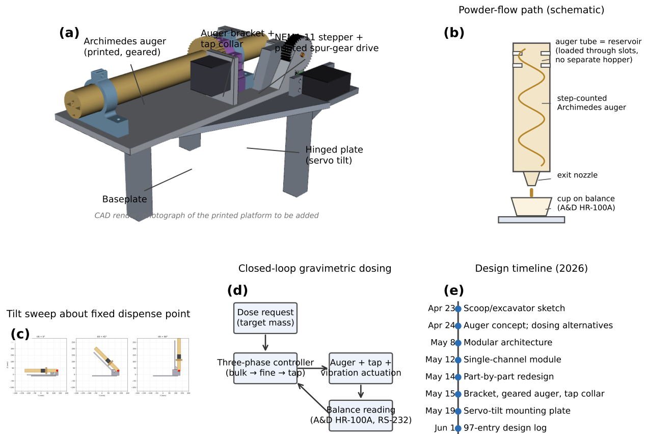
Fig. 1 Platform overview. (a) Single-channel powder-doser module (CAD render; photograph of the printed platform will replace this render): printed Archimedes auger (25 mm OD), printed spur-gear drive from a NEMA-11 stepper, tap collar (which mounts the tap solenoid and ERM vibration motor, not individually resolved at this scale), and servo-tilted hinged mounting plate on the baseplate. (b) Schematic of the powder-flow path through the module: powder is loaded through slots into the auger tube, which is itself the reservoir (no separate hopper), and is conveyed down the helical channel → exit nozzle → collection cup on the analytical balance. (c) Tilt sweep about the fixed dispense point (red marker): the hinge axis passes through the exit-nozzle tip so the dispense point does not translate as the channel tilts from 0° (horizontal park) to 90° (vertical dispense). (d) Closed-loop gravimetric dosing concept: the target mass enters the controller, which drives the actuation while the balance feeds the measured mass back. (e) Compressed design timeline; the complete 97-entry design log (DESIGN-LOG.md) is available in the repository. Throughout, humans selected the architecture and reviewed, printed, and tested every part, while AI coding agents generated the parametric CAD models and renders; no GUI CAD package (e.g. Fusion 360, SolidWorks) was used.
