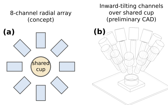
Fig. 5 Future work: multi-powder doser. (a) Eight-channel radial array concept (schematic) around a shared collection cup. (b) Preliminary programmatic-CAD study of inward-tilting channels over the shared cup. As elsewhere, the concept was set by the human team and the CAD modelled by AI coding agents; no GUI CAD package was used.
