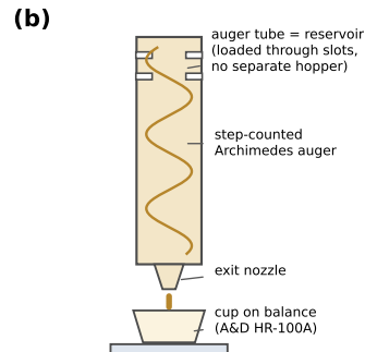
Powder-flow path (schematic)
