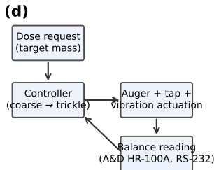
Closed-loop gravimetric dosing
