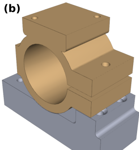
Tap collar split clamp (actuator mount)
