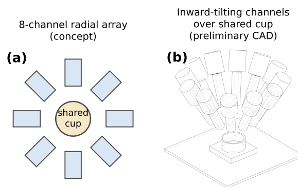
Fig. 6 Future work: the first multi-powder doser concept. (a) Eight channels arranged radially around a shared collection cup. (b) Preliminary CAD study of channels tilting inwards over the shared cup. The team set the concept and AI coding agents produced the CAD. The current multi-doser design moves passive auger cartridges on a roller chain past one fixed actuation and weighing station instead (repository issue #128).
