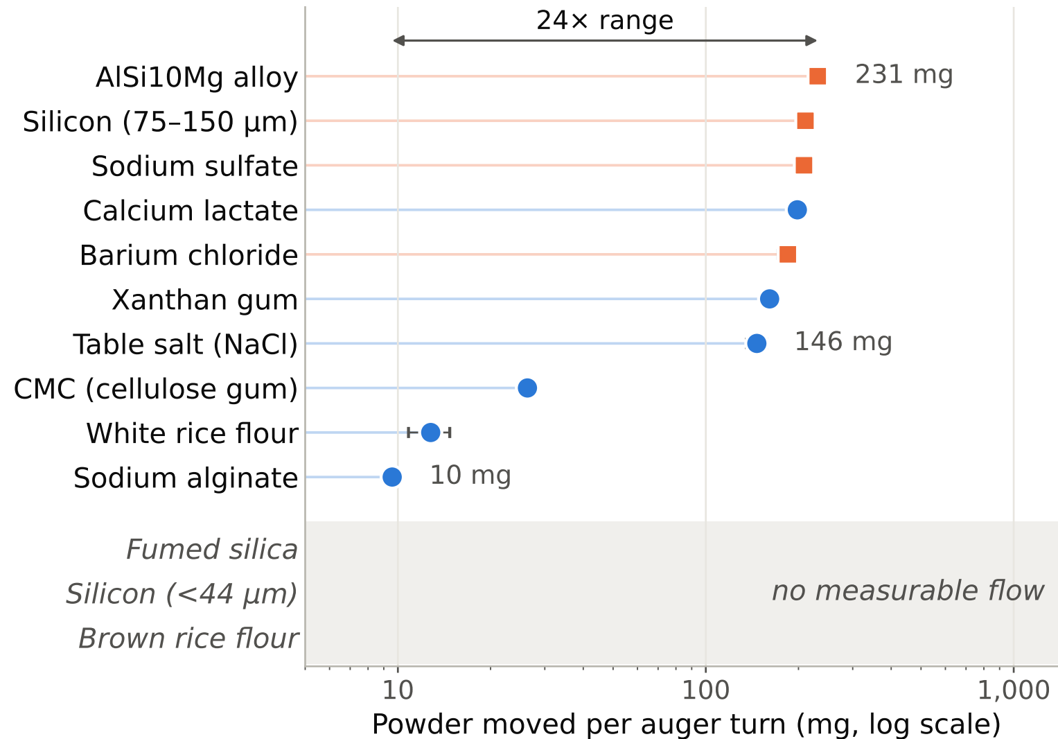
How much one turn of the auger moves
