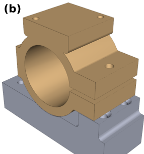
Tap collar + solenoid mount (split clamp)
