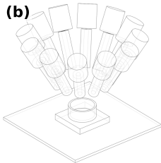
Inward-tilting channels over shared cup (CAD)
