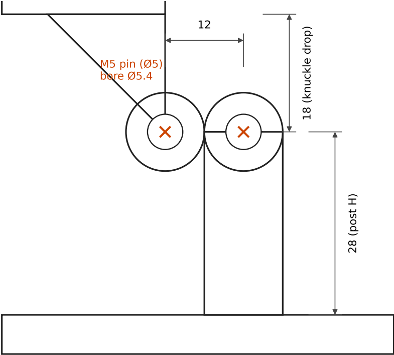
Hinge detail — SIDE view (X out of page)
