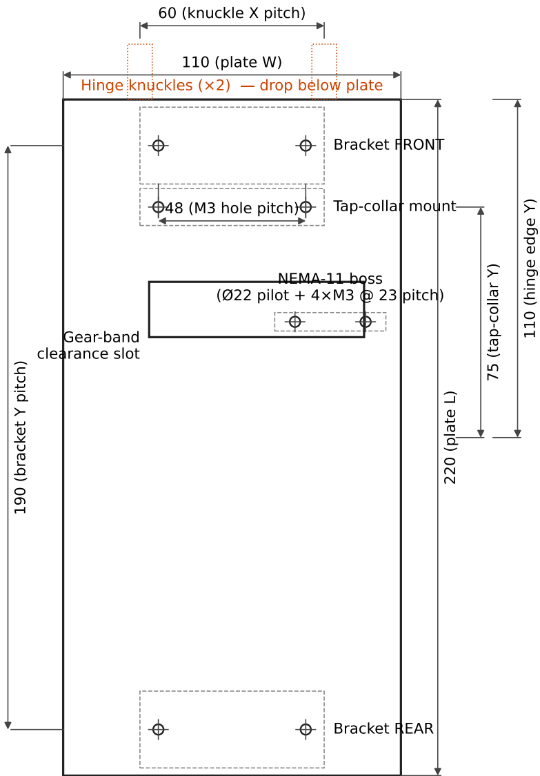
Mounting plate — TOP view (Z up out of page)
