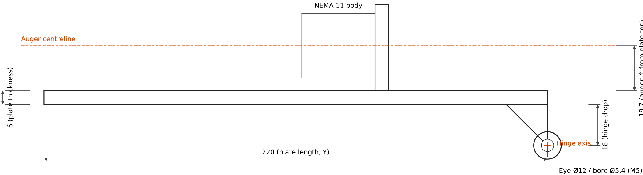
Mounting plate — SIDE view (looking along +X, Y →, Z ↑)
