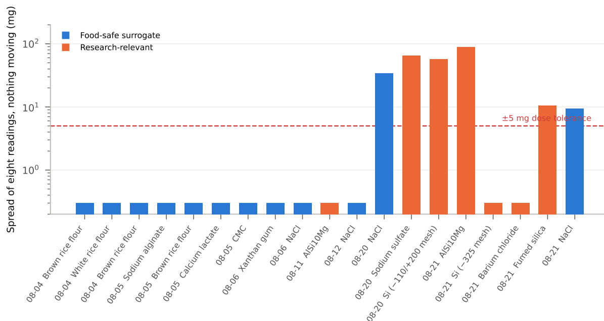
Figure S5: Balance noise floor for every first-round run: the spread (maximum minus minimum) of eight readings taken with nothing moving (protocol A), in date order. Runs whose eight readings were identical are drawn at the axis floor. The dashed line is the controller's \pm 5 mg stopping band.
