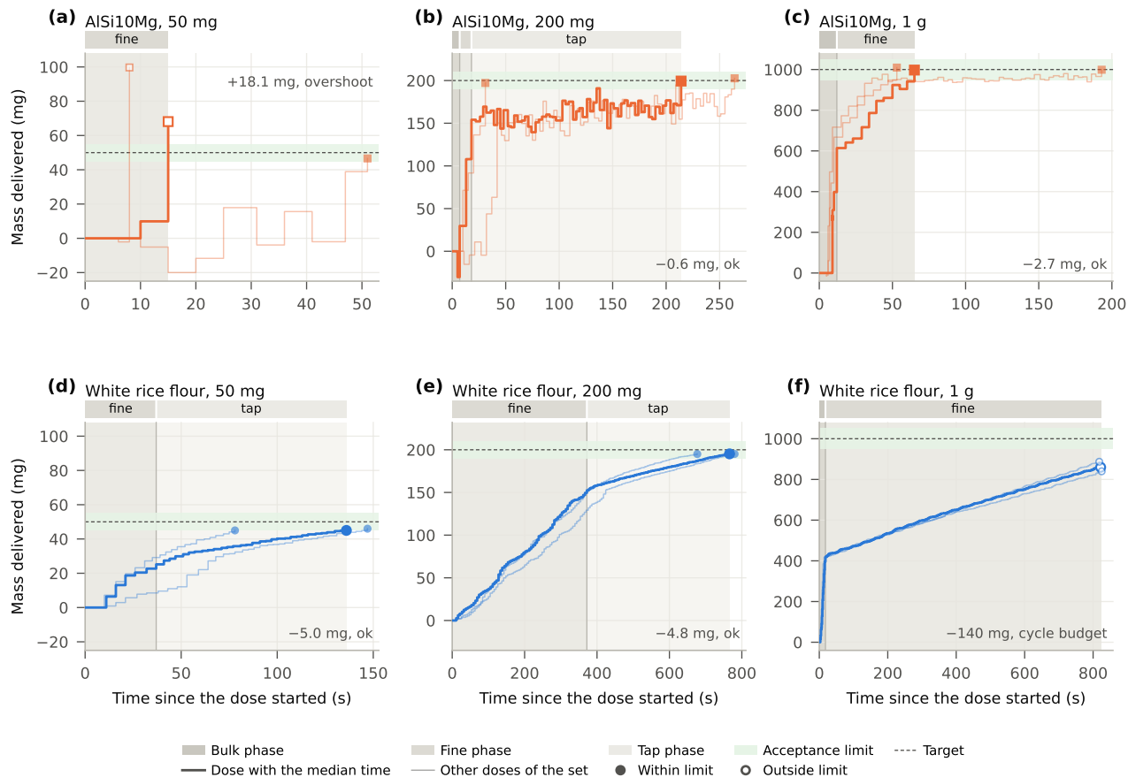
Figure S7: Balance readings during closed-loop doses of a fast, free-flowing powder (a–c, AlSi10Mg) and a slow one (d–f, white rice flour) at 50 mg, 200 mg, and 1 g. The thick line is the dose with the median time of its set of three, and thin lines are the other two. Shading and the bar above each panel mark the phases of the thick-line dose: bulk (continuous rotation, tube at 45°), fine (45° auger turns, tube at 22.5°), and tap (pairs of taps, tube horizontal). The green band is the acceptance limit and the dashed line the target. Markers are filled within the limit and open outside it. Time axes differ. In (a), the second 45° turn added 58 mg, more than the whole target. In (b), a first reading just below zero triggered a brief bulk spin. Tap-phase readings then ranged over 140–191 mg, and the dose stopped on the first reading inside the \pm 5 mg band. Panels (a–e) are from September 2026, and (f) is from 4 August 2026.
