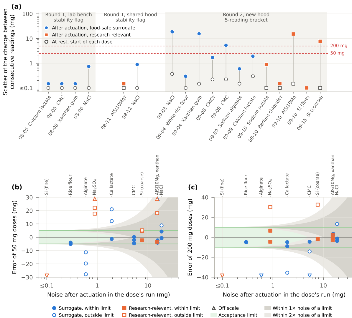
Figure S6: Balance noise after actuation and the pass/fail calls of small doses. (a) Filled markers: noise after actuation for every run with a closed-loop tap phase, the robust standard deviation of the change between consecutive tap-phase readings, each taken 1.5 s after two solenoid taps with the tube horizontal. Open markers apply the same statistic at rest, to the first reading of each dose minus its tare reading. Fine silicon and barium chloride never reached the tap phase, so their values come from fine-phase steps that delivered nothing. Values below 0.1 mg are drawn at 0.1 mg, and † marks runs excluded from the dose analysis. Above the dashed lines, no 50 mg or 200 mg dose can be a robust pass. (b, c) Error of each valid 50 and 200 mg dose against the noise of its run (named along the top). Light and dark grey zones lie within two and one times the noise of a limit. Markers as in Fig. 5 of the main text.
