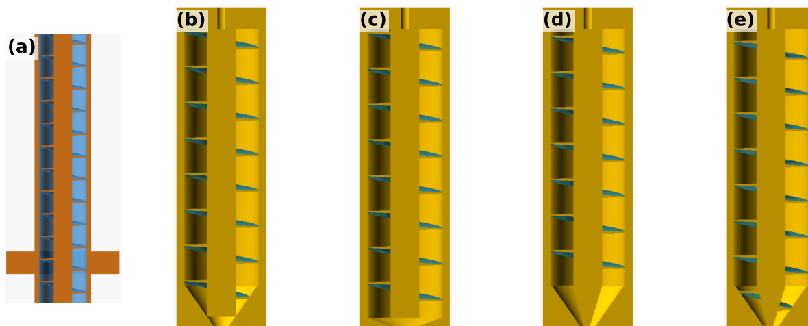
Figure S3: (a) Cross-section of the AI-modelled geared auger: the 8 mm central core, the single-start helical flight (10 mm pitch) running the full length of the 21 mm bore, and the external gear band. (b–e) Cross-sections of the four outlet variants (Types 1–4), which differ in exit constriction and chamfer. All are parametric OpenSCAD models ( cad/auger-geared/ in the repository) written by AI coding agents under human review; no conventional CAD software was used to design them. The auger used in the tests is the team's later Fusion 360 part (main text, Fig. 1c). Its flight is 0.5 mm thick with a 10.4 mm pitch and covers only the third of the tube nearest the outlet, the tube is filled through a screw-on cap rather than through loading slots, and its gear has 44 teeth rather than 48 (Table S3).
