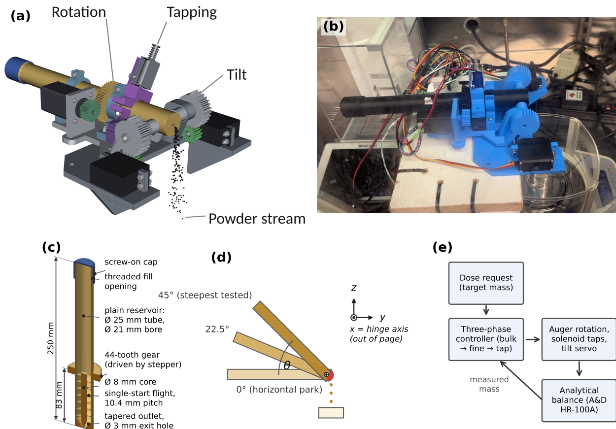
Fig. 1 The single-channel powder doser. (a) Annotated CAD model of the current design, showing the three motions used in this work: auger rotation, tapping, and tilt. Every printed part in this model is the team's Fusion 360 part except the tap-collar base, which is still the AI-modelled part. The stepper, servos, and solenoid are simplified models made from their datasheets (SI Figs. S1 and S2 show every part). (b) The module as built, photographed from the same viewpoint during its first automated dispense (sodium chloride into a crucible on the balance), inside a glove box at the University of Utah. The tests reported here were run on an open bench and in fume hoods. (c) Cut-away rendering of the tested auger and its screw-on cap, cut in half through the tube axis and drawn upright (outlet at the bottom). Cut faces are the flat, darker areas. The tube is itself the reservoir and is filled through the capped end. The flight and its core fill only the 83 mm nearest the outlet, and the 44-tooth gear is printed on the outside. Tube, flight, core, and gear are one printed piece and turn together. (d) Tilt about the hinge axis x , which runs about 12 mm behind the outlet (red), so the dose lands in nearly the same place as the tilt angle \theta changes from 0° (horizontal park) to 45°, the steepest tilt used in this work. (e) Closed-loop dosing: the three-phase controller (bulk, then fine, then tap) compares the requested mass with the balance reading and drives the actuators until the two agree. Humans made every design decision and reviewed, printed, and tested every part. AI tools produced the original CAD models without conventional CAD software, and the team later recreated every printed part except the tap-collar base in Fusion 360.
