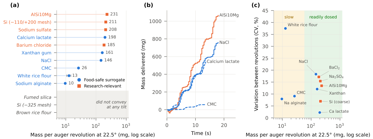
Fig. 3 How much powder the auger delivers, for 13 powders under one fixed set of settings. (a) Mass delivered per auger revolution at 22.5° tilt (protocol C, six revolutions at 30 rpm, with standard-error bars). The three powders at the bottom delivered nothing distinguishable from zero at any tilt and are listed without a value. (b) Balance readings streamed while the auger turned continuously at 15 rpm and 22.5° tilt (protocol D), for four powders. The mass rises in steps about 4 s apart, one per auger revolution. (c) Mass per revolution against the variation between successive revolutions (coefficient of variation of six revolutions). Both numbers come from protocol C alone. The shading marks the two groups discussed in the text. Blue circles are food-safe surrogates and orange squares research-relevant powders. One run per powder is shown (see Experimental). Fill level was not controlled, particle size and shape were not measured, and all research-relevant powders were tested in the noisier period. Rotations and speeds refer to the auger, and angles to the tube's tilt above horizontal.
