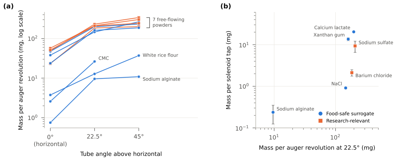
Fig. 4 Effect of tilt and tapping. (a) Mass per auger revolution with the tube horizontal and tilted to 22.5° and 45° (protocol C) for the ten powders that conveyed a measurable amount. A point is shown only when its mean is more than twice its standard error, that is, clearly larger than the scatter. CMC at 45° did not meet this rule. The seven free-flowing powders overlap at the top and are bracketed, and Table 2 gives their values. On the logarithmic axis, equal vertical distances are equal ratios. (b) Mass released by one solenoid tap (protocol E, mean and standard error of eight taps at 22.5°) against mass per auger revolution, CMC, for the six powders whose tap increment exceeded twice its standard error. Markers as in Fig. 3.
