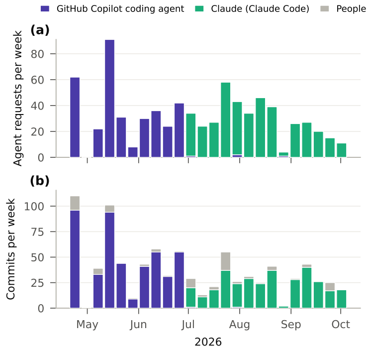
Figure S7: Generative-AI agent activity per week over the project. (a) Requests to an agent: comments and issue or pull-request descriptions written by a team member that address @copilot or @claude, plus pull requests the Copilot coding agent opened when assigned an issue. Most such requests started one agent session, so the count is an approximate measure of use. (b) Commits on all branches by author; commits that were later rebased onto another branch are counted once. Counts are from the public repository history ( paper/figures/data/build_ai_usage.py ).
