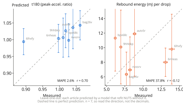
Fig. 8 Round-1 leave-one-out cross-validation of the SAASBO surrogate: predicted versus observed values with model error bars for both objectives.
