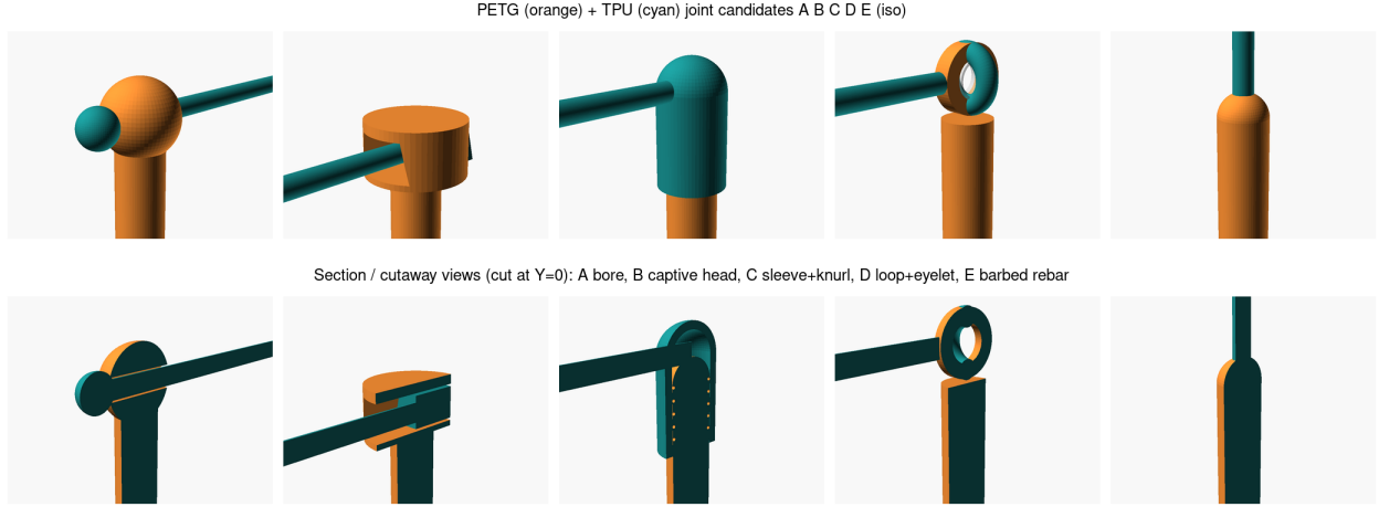
Figure S1: Five candidate strut-to-cable joint geometries from the OpenSCAD joint study (left to right: A anchor-bulb, B dovetail, C TPU-sleeve overmold, D eyelet-loop, E TPU-rebar; top row isometric, bottom row section views). The study renders use the PETG (orange) + TPU (cyan) material pair under which the joint family was first developed; the working prototype adapts the selected dovetail (B) with an anchor-bulb (A) backup to the PLA/TPU pair of the main text, with the captive TPU core routed inside the PLA shell.
