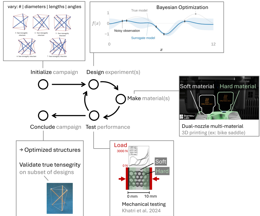
Fig. 1 Closed-loop, experiment-driven design framework. Parameterized PLA/TPU tensegrity-inspired unit cells are printed, tested under quasi-static compression and drop-weight impact, and the resulting performance data drive a Gaussian-process surrogate that recommends the next batch of designs to fabricate.
