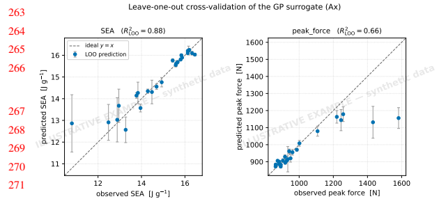
Fig. 5 Illustrative example (synthetic data). Leave-one-out cross-validation of the Gaussian-process surrogate—predicted vs. observed specific energy absorption (SEA) and peak transmitted force, with model error bars and R^2_{LOO} —obtained from a real Ax/BoTorch run on synthetic objective values. To be regenerated from campaign data.
