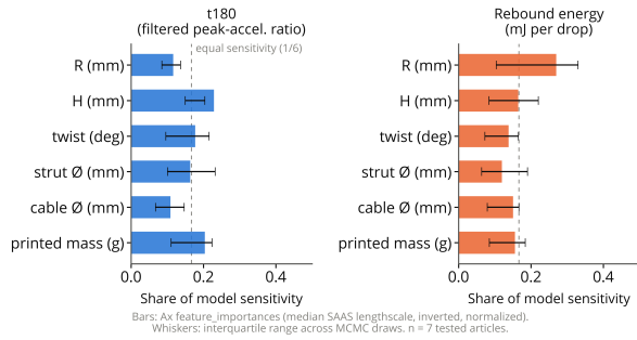
Fig. 8 Round-1 SAASBO length-scale diagnostics per objective (normalized inverse length scales; median over MCMC draws, interquartile whiskers; inputs are the five design variables plus printed mass; the horizontal axis, labeled “share of model sensitivity” in the plot, is this normalized inverse-length-scale diagnostic). No input separates decisively from the equal-share line (dashed) at seven mapped articles, and these are prior-sensitive model diagnostics, not evidence of variable relevance.
