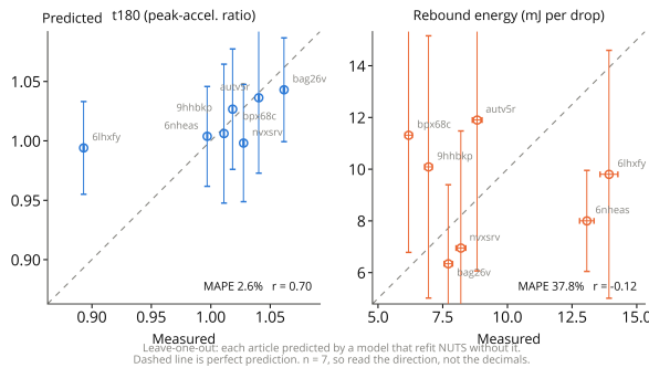
Fig. 9 Round-1 leave-one-out cross-validation of the SAASBO surrogate: predicted versus observed values with model error bars for both objectives.
