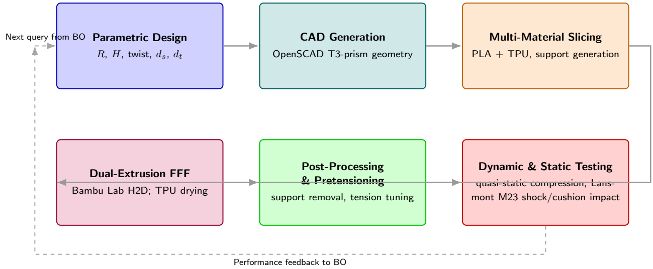
Fig. 3 Fabrication and characterization workflow for the multi-material tensegrity-inspired unit cells: design parameters drive parametric CAD, slicing with manually generated TPU supports, a single multi-material print on the Bambu Lab H2D, post-processing and inspection, and mechanical testing.
