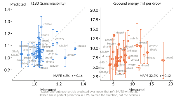
Fig. 9 Leave-one-out cross-validation of the SAASBO surrogate on the 26 articles of batches 1 to 3 (one full NUTS refit per held-out article; 12 model inputs). Vertical bars are one posterior standard deviation of the held-out prediction; horizontal bars are the measured standard error as ingested. The dashed line is parity. The held-out posterior shrinks toward the pooled mean, so the extremes (r2d2c3, drran7, the seed attenuator) are the largest misses.
