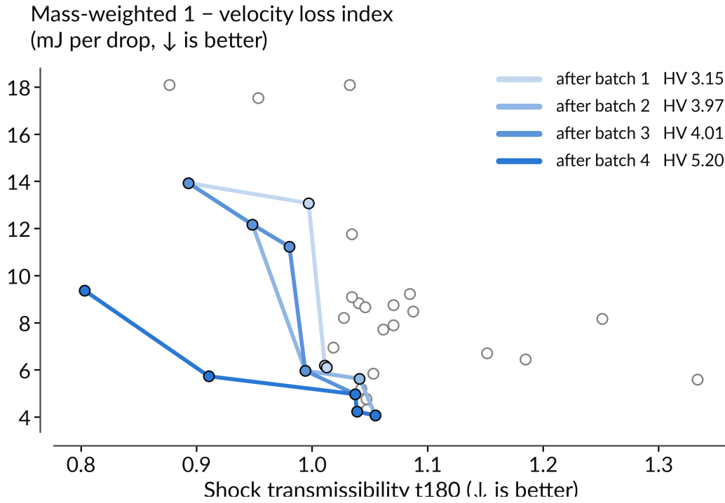
Fig. 6 Measured objective space and front evolution across the four batches; the vertical axis is the mass-weighted velocity-loss objective E_{reb} = (1 - VLI) mgh of Eq. (1). Gray circles are all measured articles at their stabilized means; the blue lines are the non-dominated fronts after each batch, with the dominated hypervolume at the (1.35, 15 mJ) reference in the legend. Batch 2 grew the front on the velocity-loss axis, batch 3 filled the knee, and batch 4 broke the transmissibility floor. Repeated batch-3 designs are drawn at their first-print values; the design-mean front is given in the text. Both axes improve downward.
