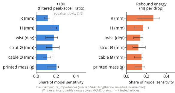
Fig. 8 Round-1 SAASBO feature importances per objective (normalized inverse length scales; median over MCMC draws, interquartile range across MCMC draws, inverted, normalized). Inputs are the five design variables plus printed mass). No input separates decisively from the equal-share line (dashed) at seven mapped articles.
