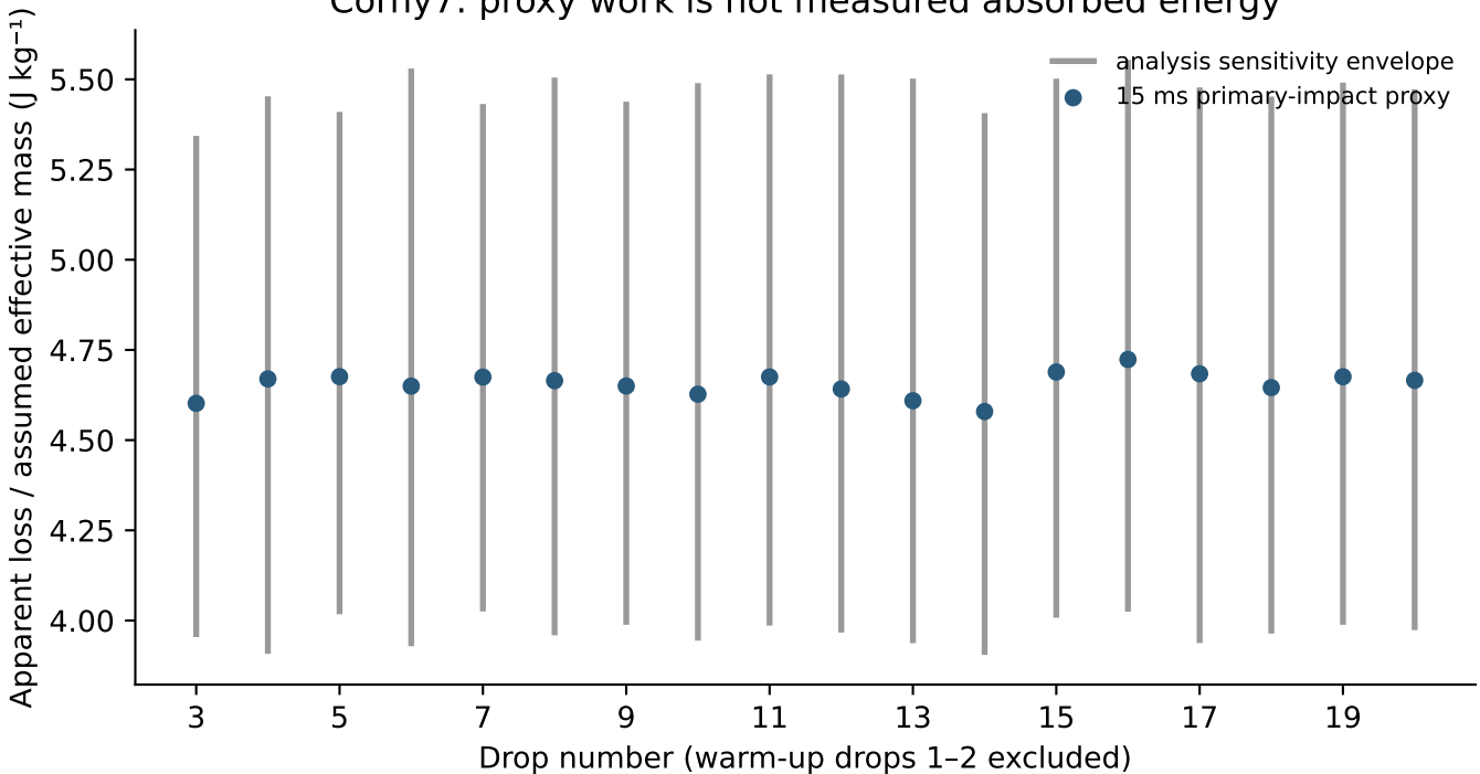
Corny7: proxy work is not measured absorbed energy
