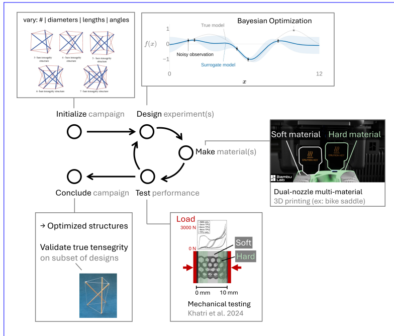
Figure 1: Research framework overview. Students design, print, and test tensegrity-inspired specimens in a closed-loop Bayesian optimization cycle that recommends the next designs to fabricate. Performance is evaluated via quasi-static compression and drop-weight impact tests.
