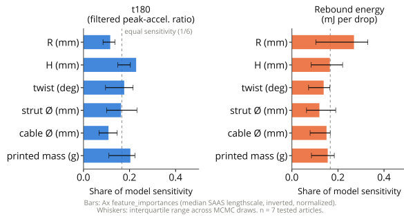
Fig. 7 Round-1 SAASBO length-scale diagnostics per objective (normalized inverse length scales; median over MCMC draws, interquartile whiskers; inputs are the five design variables plus printed mass; the horizontal axis, labeled “share of model sensitivity” in the plot, is this normalized inverse-length-scale diagnostic). No input separates decisively from the equal-share line (dashed) at seven mapped articles, and these are prior-seen model diagnostics, not evidence of variable relevance.
