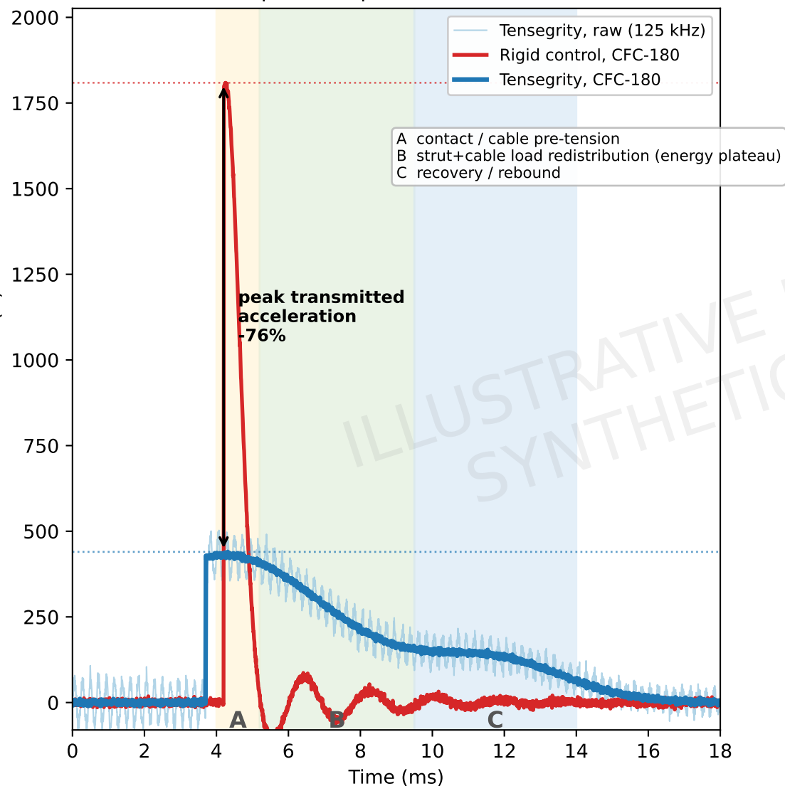
(a) Processed drop-test response
