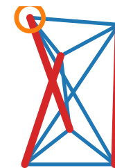
(b) Specimen under test (T3 prism)
