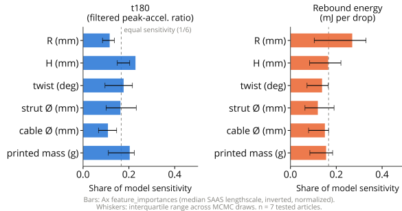
Fig. 8 Seed-state SAASBO length-scale diagnostics per objective (normalized inverse length scales; median over MCMC draws, interquartile whiskers; inputs are the five design variables plus printed mass; the horizontal axis, labeled “share of model sensitivity” in the plot, is this normalized inverse-length-scale diagnostic). No input separates decisively from the equal-share line (dashed) at seven mapped articles, and these are prior-sensitive model diagnostics, not evidence of variable relevance.
