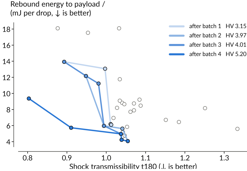
Fig. 6 Measured objective space and front evolution across the four batches. Gray circles are all measured articles at their stabilized means; the blue lines are the non-dominated fronts after each batch, with the dominated hypervolume at the (1.35, 15 mJ) reference in the legend. Batch 2 grew the front on the rebound axis, batch 3 filled the knee, and batch 4 broke the transmissibility floor. Repeated batch-3 designs are drawn at their first-print values; the design-mean front is given in the text. Both axes improve downward.
