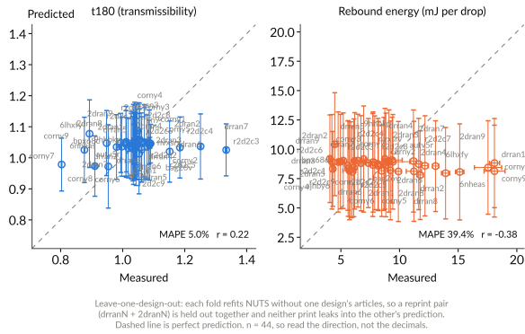
Fig. 9 Leave-one-design-out cross-validation of the SAASBO surrogate over the full 44-article record (35 design folds; each batch-3 reprint pair is held out together so neither print leaks into the other's prediction; one full NUTS refit per fold). Vertical bars are one posterior standard deviation of the held-out prediction; horizontal bars are the ingested standard error; the dashed line is parity. The held-out t_{180} posterior hugs the pooled mean (MAPE 5.0%, rank correlation +0.08) and the rebound ordering is anti-correlated (−0.38): design-level held-out skill is near zero on transmissibility and absent on rebound.
