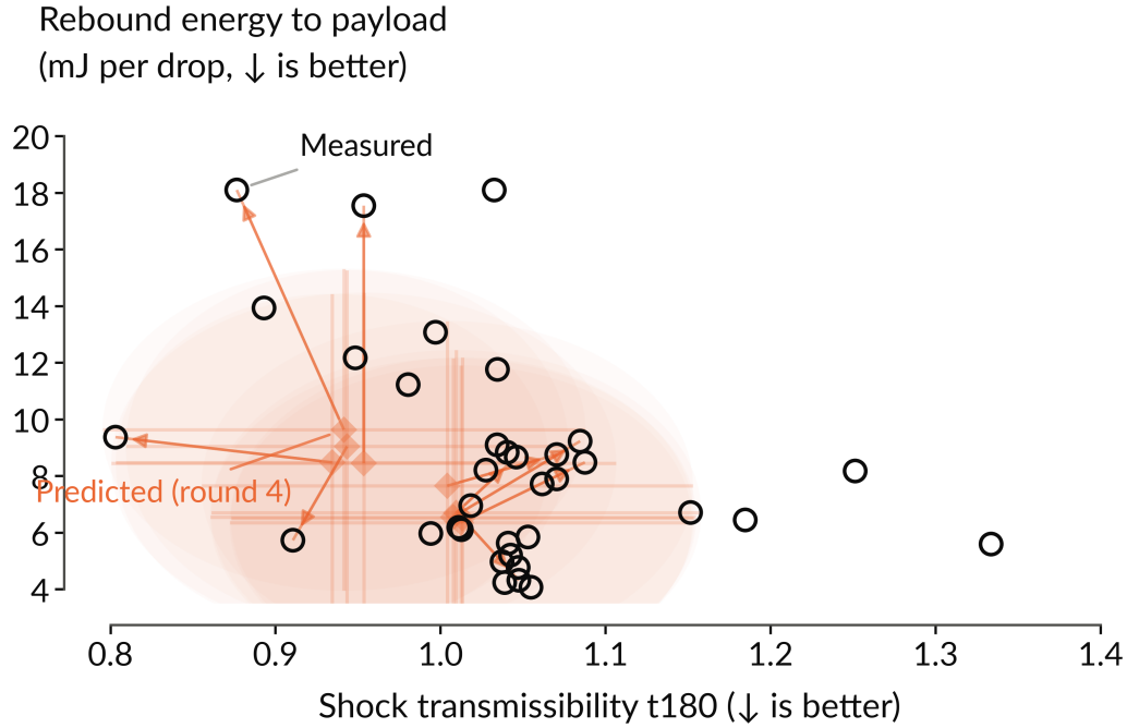
Fig. 7 Batch-4 predictions against outcomes. Orange diamonds with bars are the archived posterior predictions (mean \pm one standard deviation) for trials 37 to 45 at recommendation time; arrows connect each prediction to its article's measured value (black circles; all previously measured articles shown for context). The record attenuator corny7 (measured 0.803) is the leftmost measured point. Both axes improve downward.
